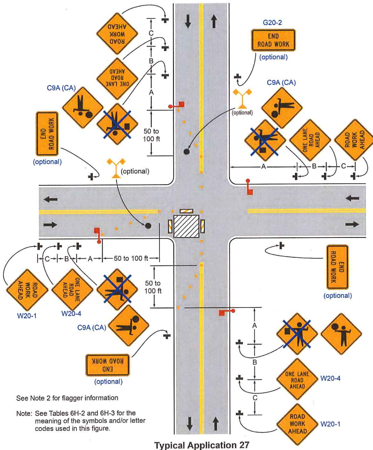
Figure 6H-27. Closure at the Side of an Intersection (TA-27) FOR USE AT CARROLTON RD AND LONE TREE RD
